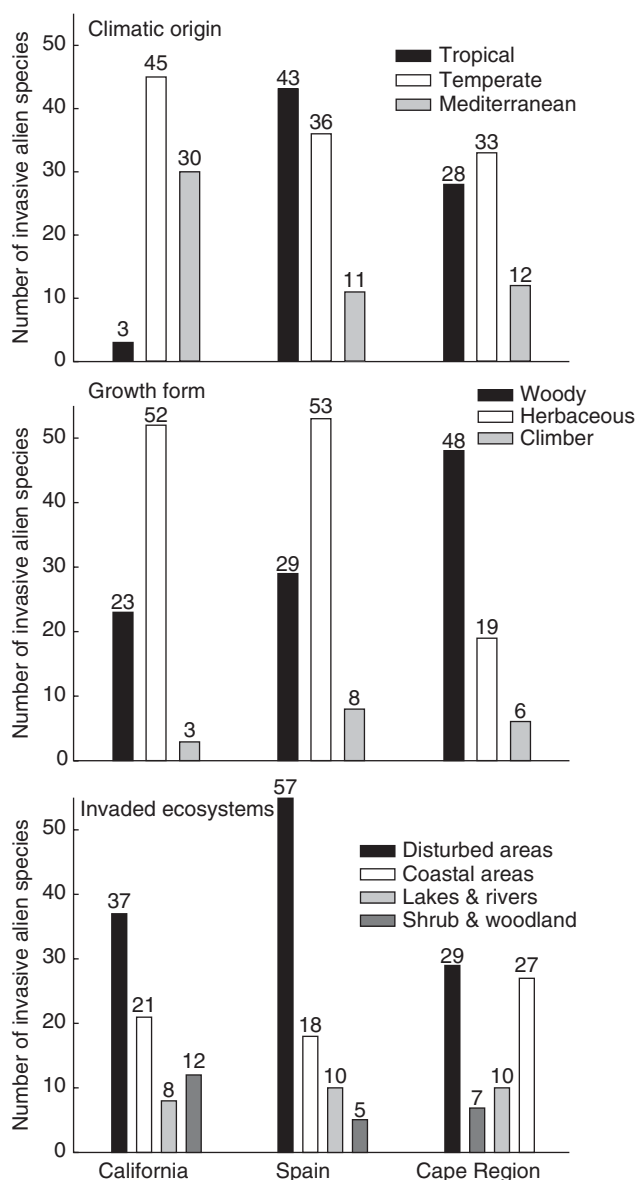
FIG. 2. Proportions of invasive species according to their climatic origin, growth form and invaded ecosystem in the three Mediterranean climate regions.
