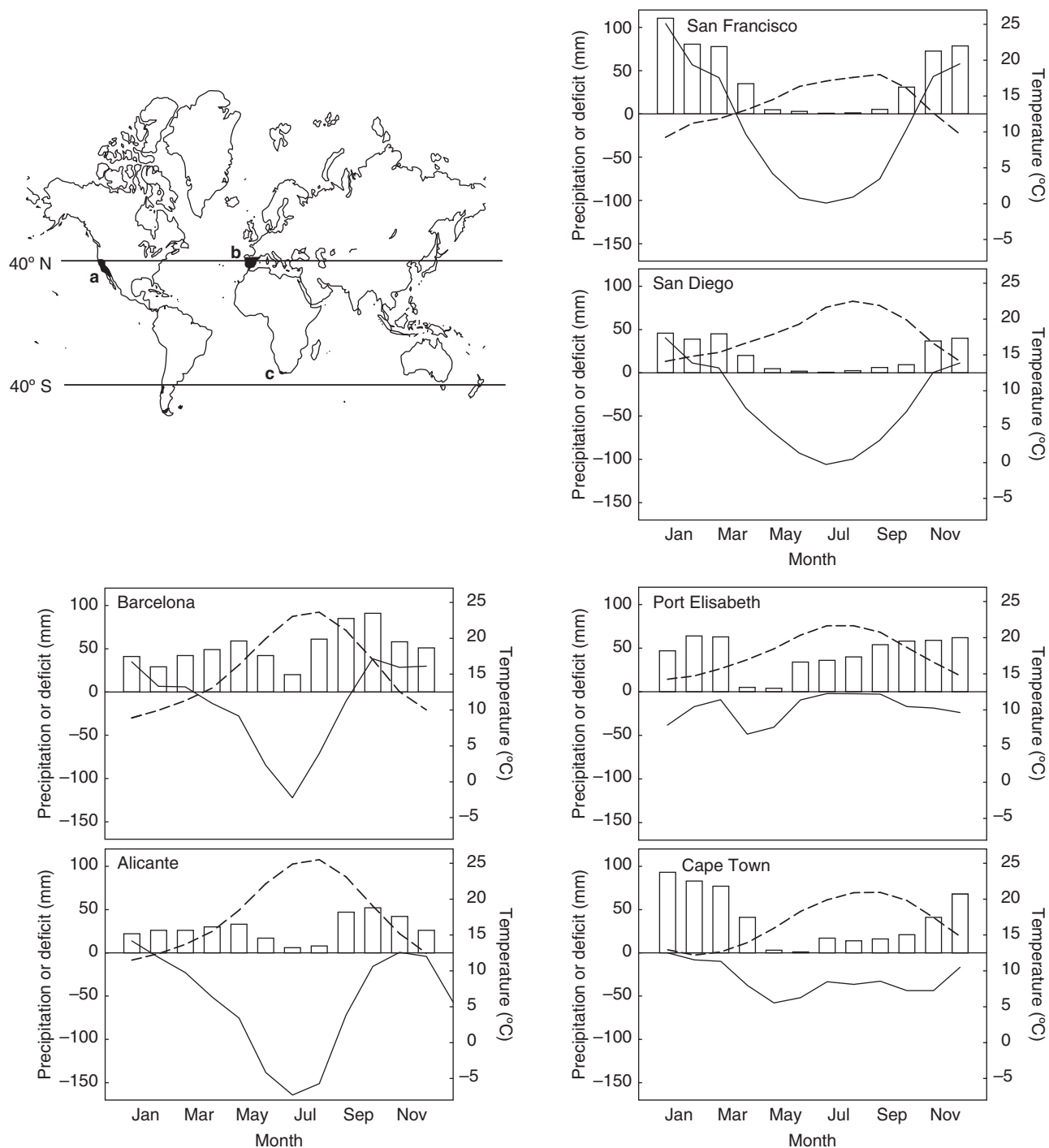
FIG. 1. Climatic characteristic of the three Mediterranean-type ecosystems studied: (a) California, (b) Spain and (c) the Cape region of South Africa. The three regions represent a gradient of summer drought severity. California has the driest and the Cape region has the mildest summers. Climatic charts of two different localities in each region illustrate this gradient. Columns represent the precipitation; solid lines the temperature; and dashed lines the water deficit in each month. Charts of the southern hemisphere localities (Cape region) have been modified to show drought between June and July for clearer comparison with Northern Hemisphere localities.
