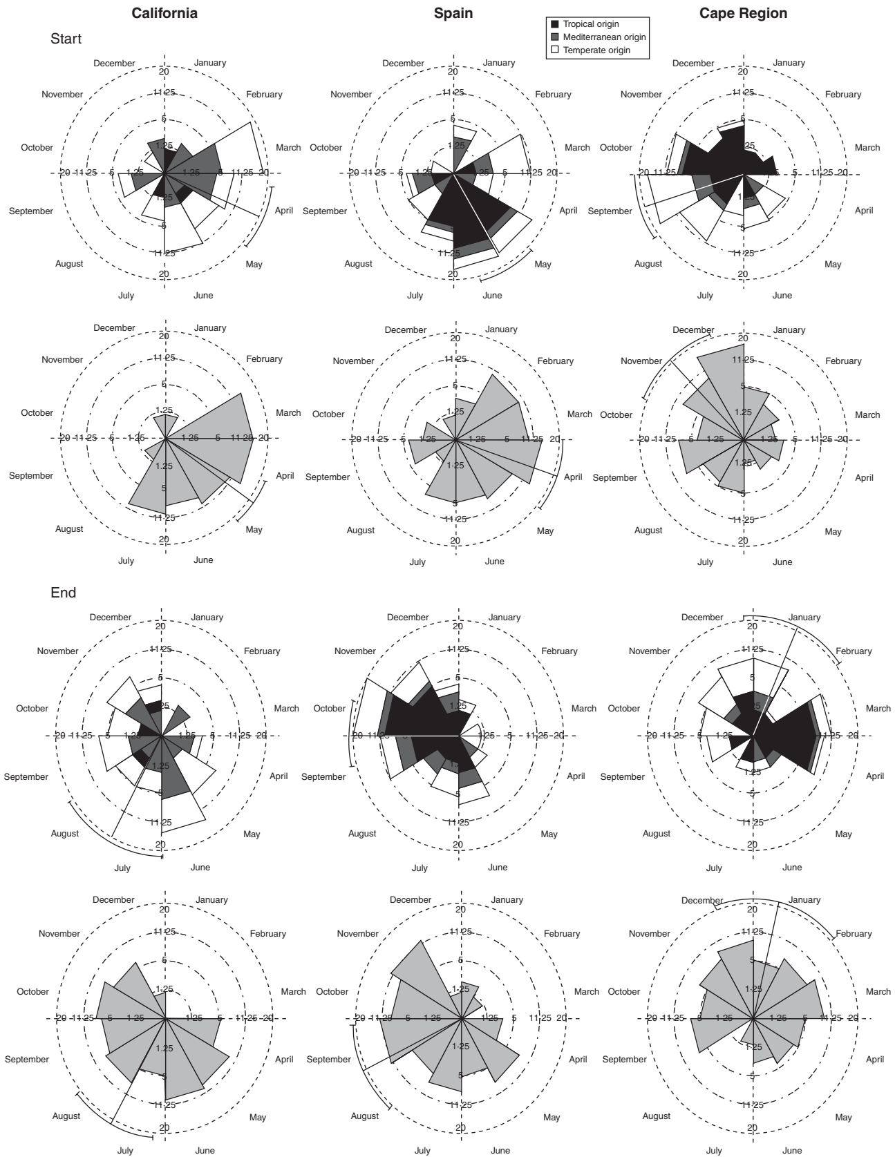
FIG. 3. Circular histograms for the start and the end of flowering in animal-pollinated invasive species and corresponding native species (see text). The triangles represent the number of species that flower in that month. Black areas indicate alien species of tropical origin; white areas indicate species with temperate origin; and dark grey areas show species with Mediterranean origin. Native species are shown separately in light grey below. Means and s.d. are also shown.
